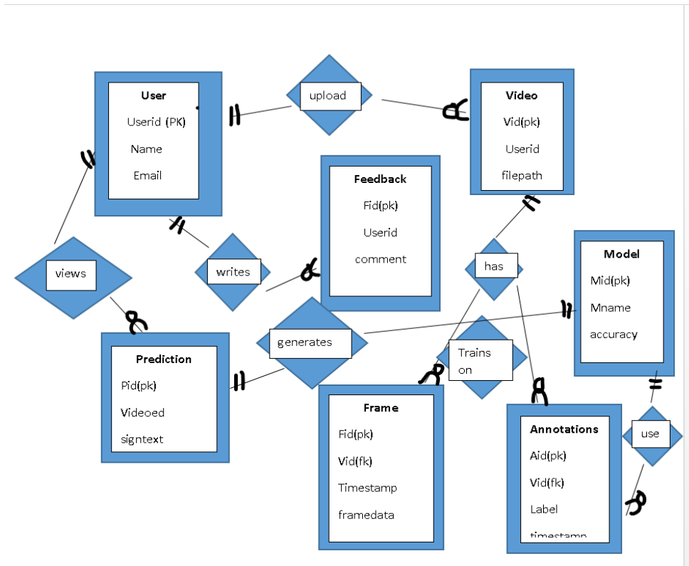
Fig. 3.3 Entity Relation Diagram
