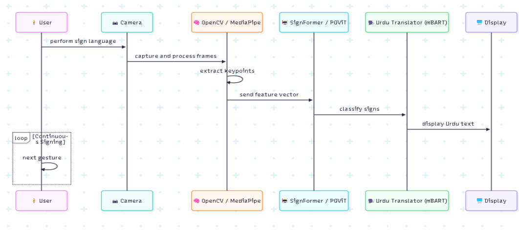
Fig 3.6 Real time translation
