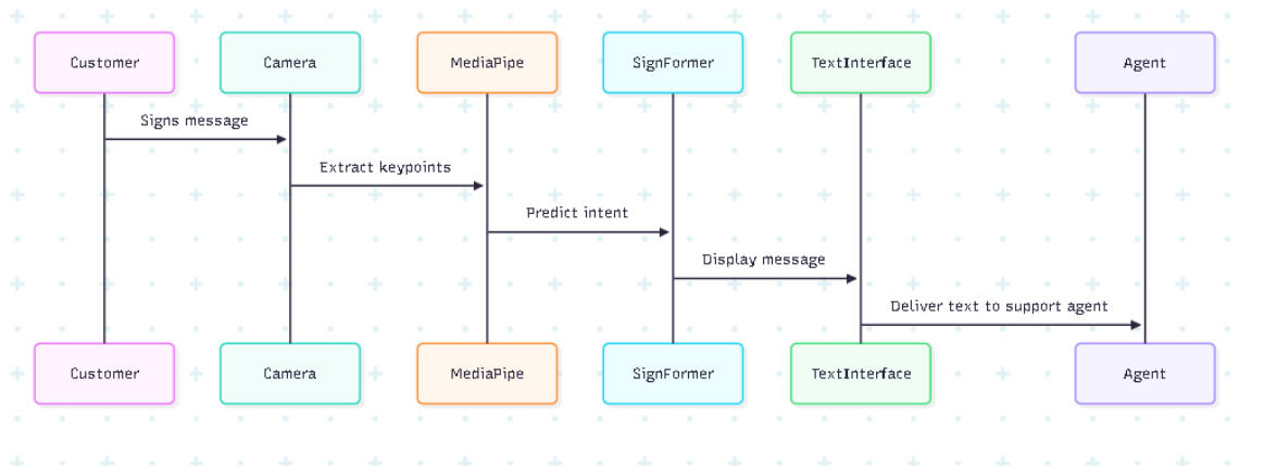
Fig. 3.9 Customer care support
