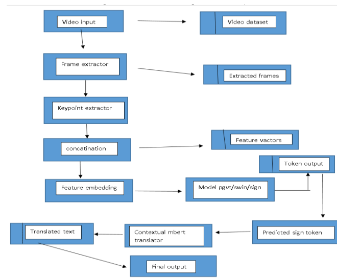
Fig. 3.5. Data Flow Diagram
