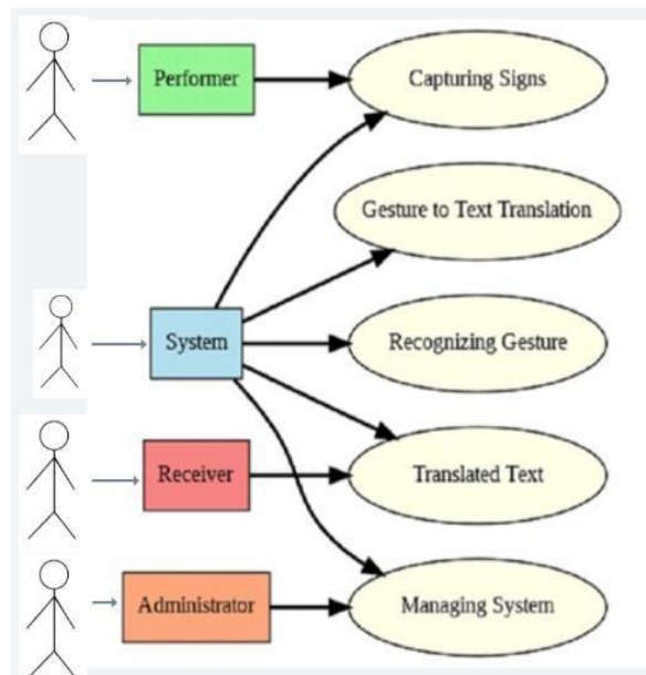
Fig. 3.2 Use Case Diagram
