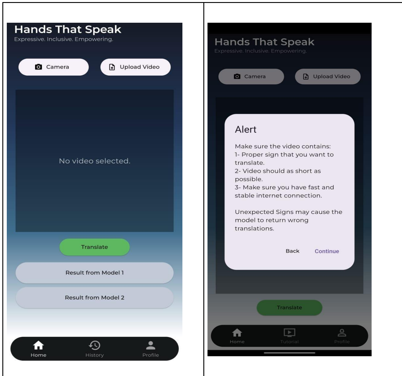
Fig.3.13. Home Screen & Fig.3.13. (b) Confirmation before translation
